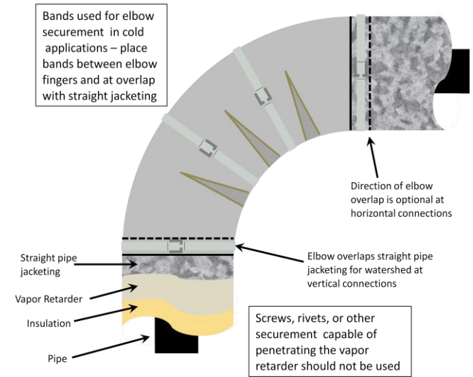
Securement of ITW Aluminum Elbow Covers in Cold Applications
